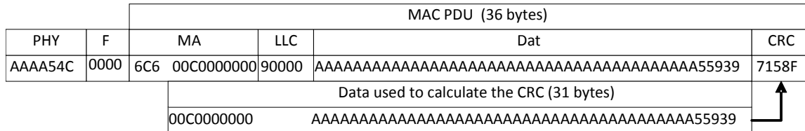
Figure 8 Example of the CRC of a MAC frame
