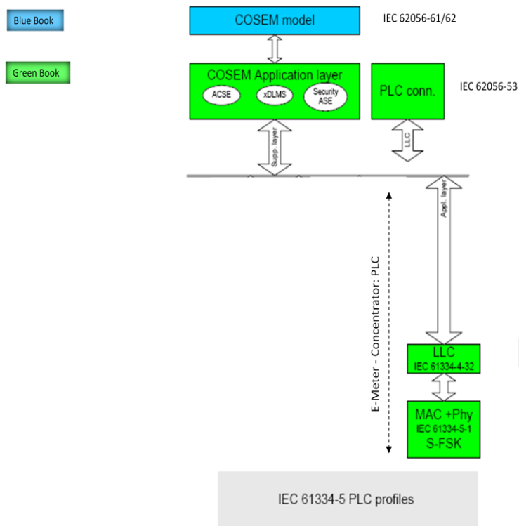
Figure 3: PLC communication supported by IDIS package 1
